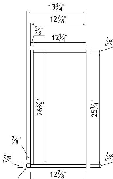
SECTION VIEW
