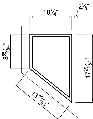
BASE DETAIL
