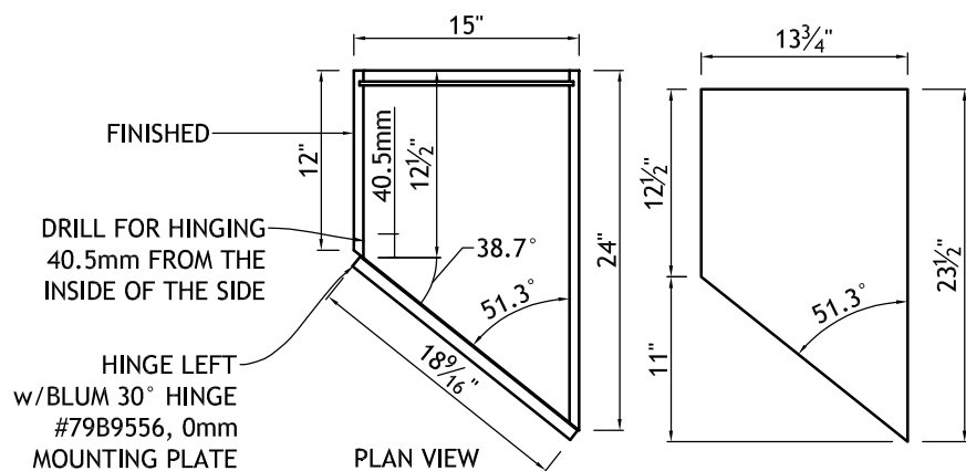
FLOOR DETAIL
