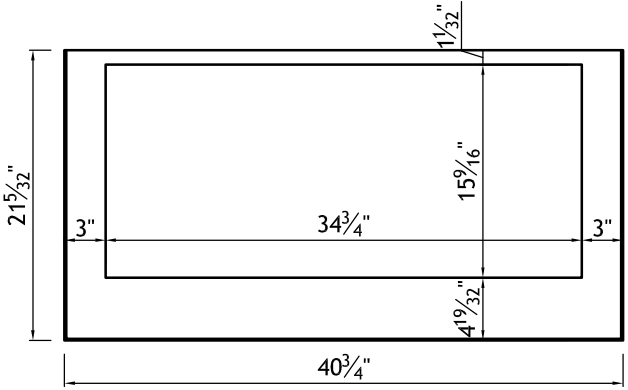
BOTTOM UPPER FLOOR DETAIL 18mm PLYWOOD
