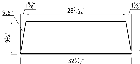
UPPER FRONT PANEL DETAIL - 9.6° TOP AND BOTTOM MITER - 44.2° COMPOUND MITER
