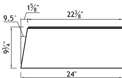
LOWER SIDE PANEL DETAIL - 9.6° TOP AND BOTTOM MITER - 44.2° COMPOUND MITER
