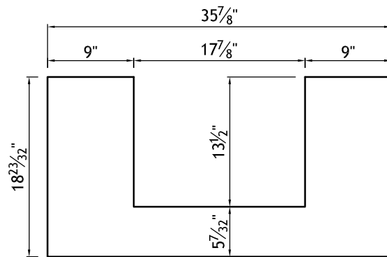
REMOVABLE SECTION MIDDLE FLOOR 18mm PLYWOOD
