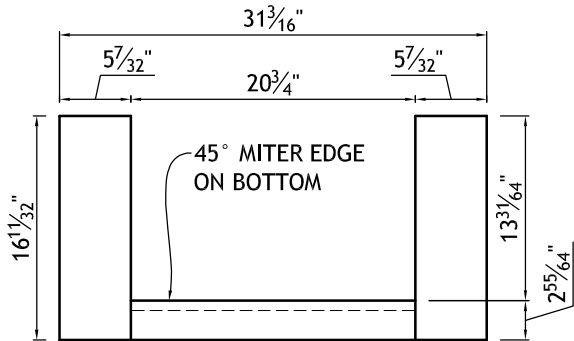
REMOVABLE SECTION TOP FLOOR 18mm PLYWOOD
