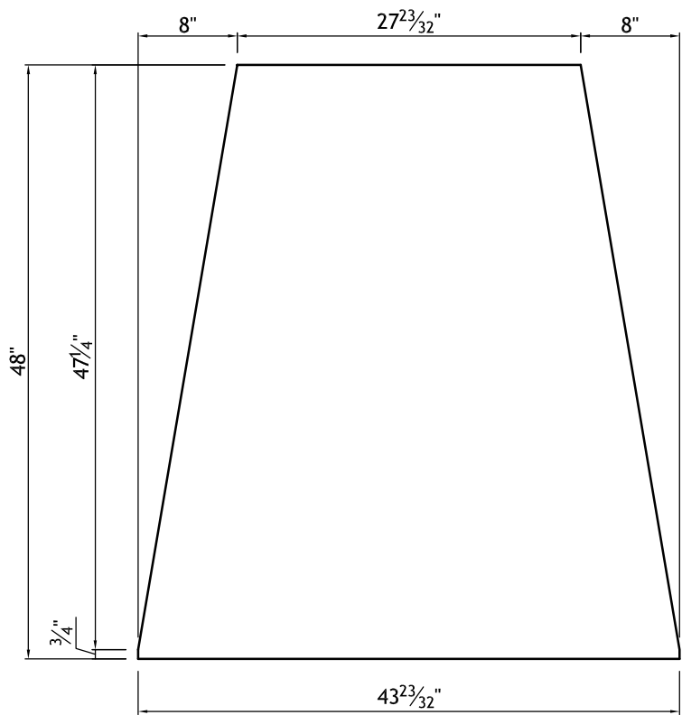
BACK DETAIL 18mm PLYWOOD
