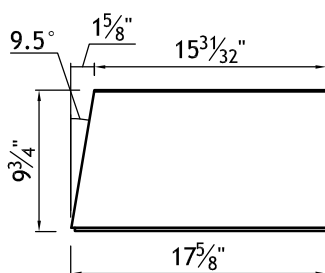
UPPER FRONT PANEL DETAIL - 9.6° TOP AND BOTTOM MITER - 44.2° COMPOUND MITER
