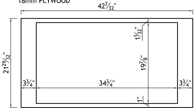
LOWER FLOOR DETAIL 18mm PLYWOOD
