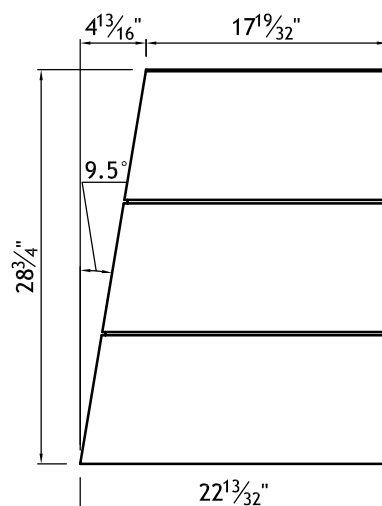
REMOVABLE SIDE PANEL DETAIL - 9.6° TOP AND BOTTOM MITER - 44.2° COMPOUND MITER
