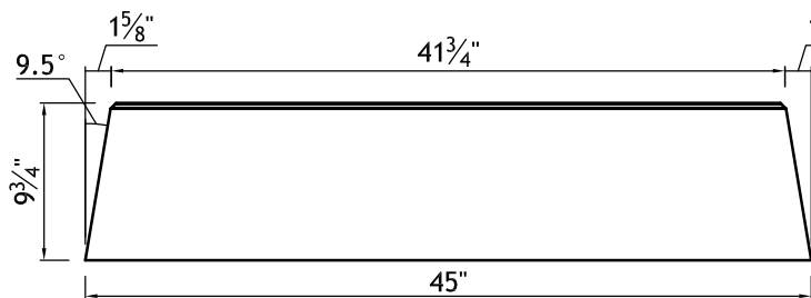
LOWER FRONT PANEL DETAIL - 9.6° TOP AND BOTTOM MITER - 44.2° COMPOUND MITER
