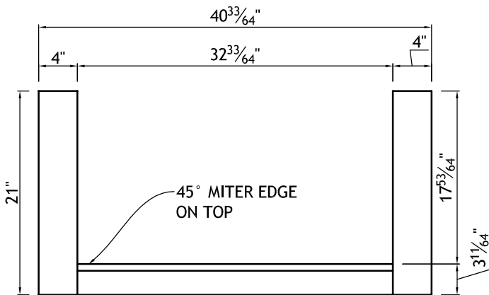
REMOVABLE SECTION BOTTOM FLOOR 18mm PLYWOOD
