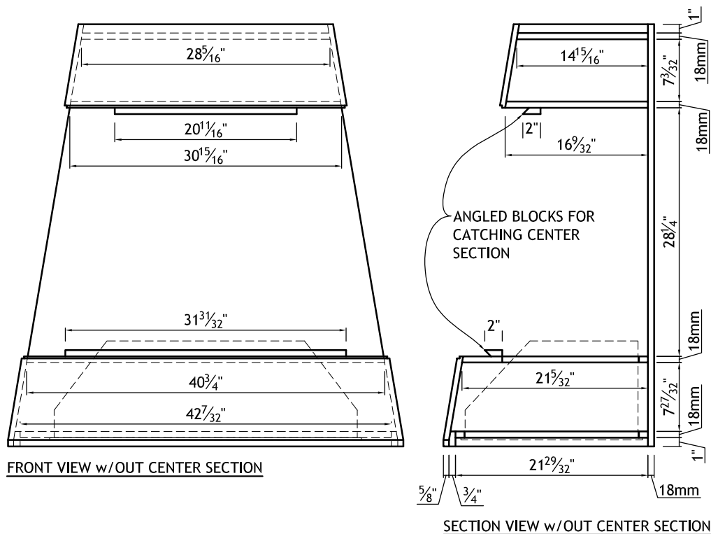
DRAWING 2 OF 5 - HOOD CABINET WITHOUT REMOVABLE CENTER SECTION
