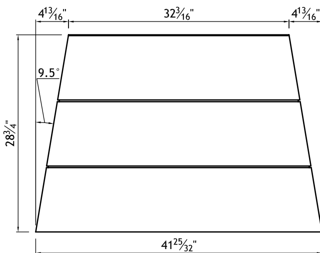
REMOVABLE FRONT PANEL DETAIL - 9.6° TOP AND BOTTOM MITER - 44.2° COMPOUND MITER
