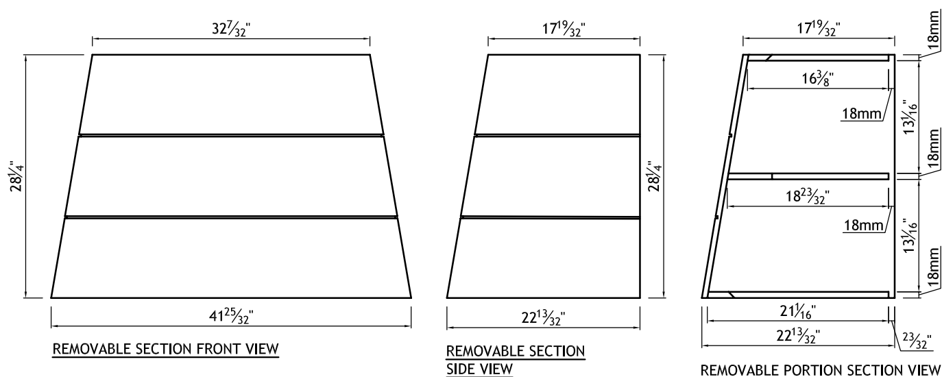
- REMOVABLE SECTION DETAIL
