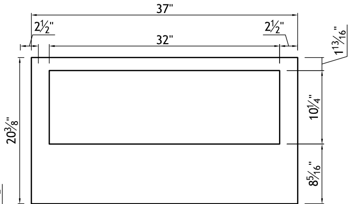
LOWER FLOOR CUT-OUT DETAIL
