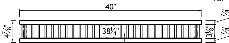
FRONT VIEW
