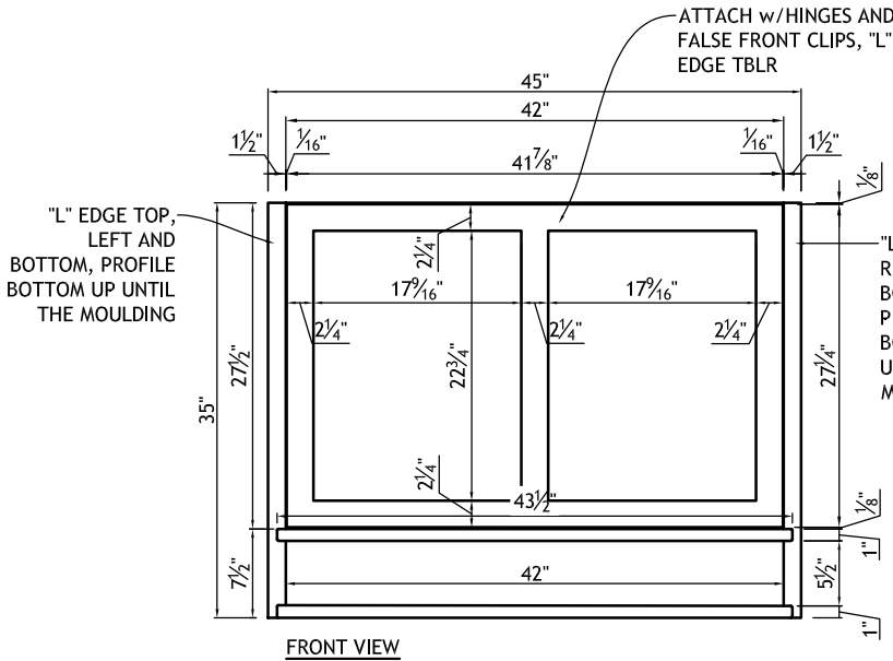
FRONT VIEW
