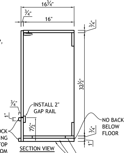
SECTION VIEW
