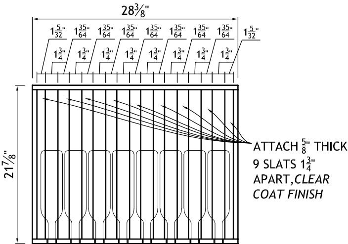
POSMDT PLAN VIEW
