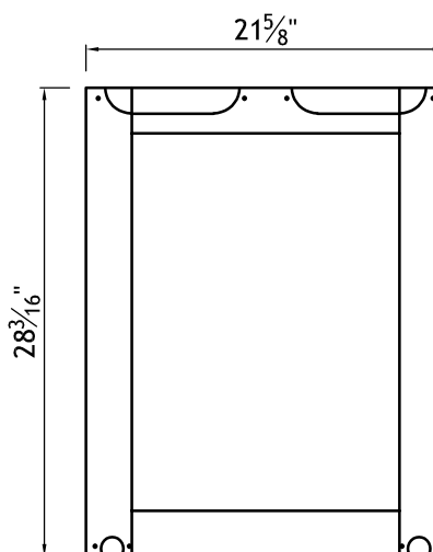
BACK VIEW OF RIGHT DOOR
