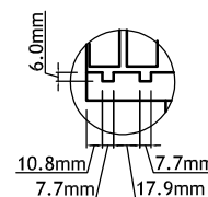
DETAIL A TOP FLOOR ALSO GROOVED FOR TRACKS(MIRRORED)
