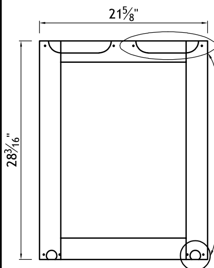
BACK VIEW OF LEFT DOOR
