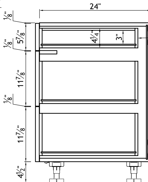
SECTION VIEW
