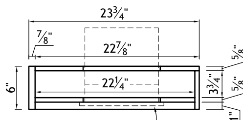
SECTION VIEW
