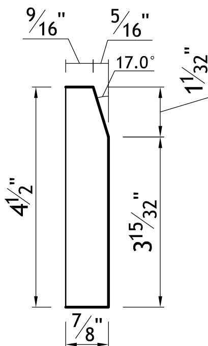
END VIEW
