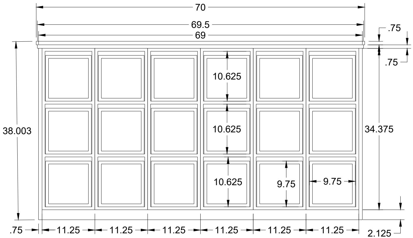
FRONT VIEW
